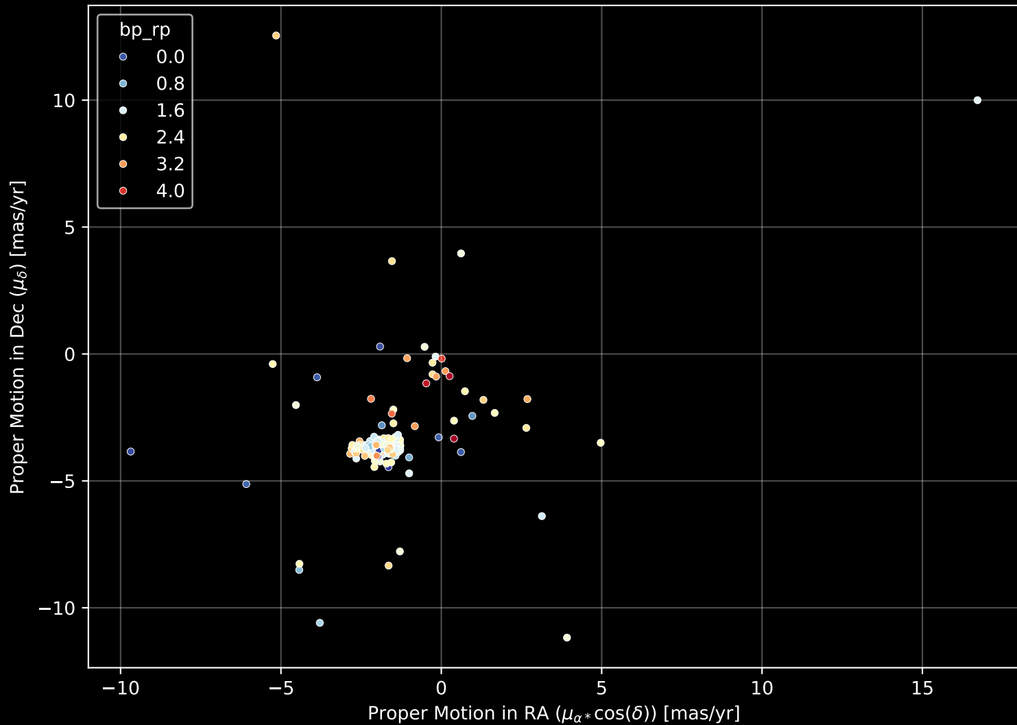
APOGEE DR17 Field: [N2264] Proper Motion Diagram (n= 152)
