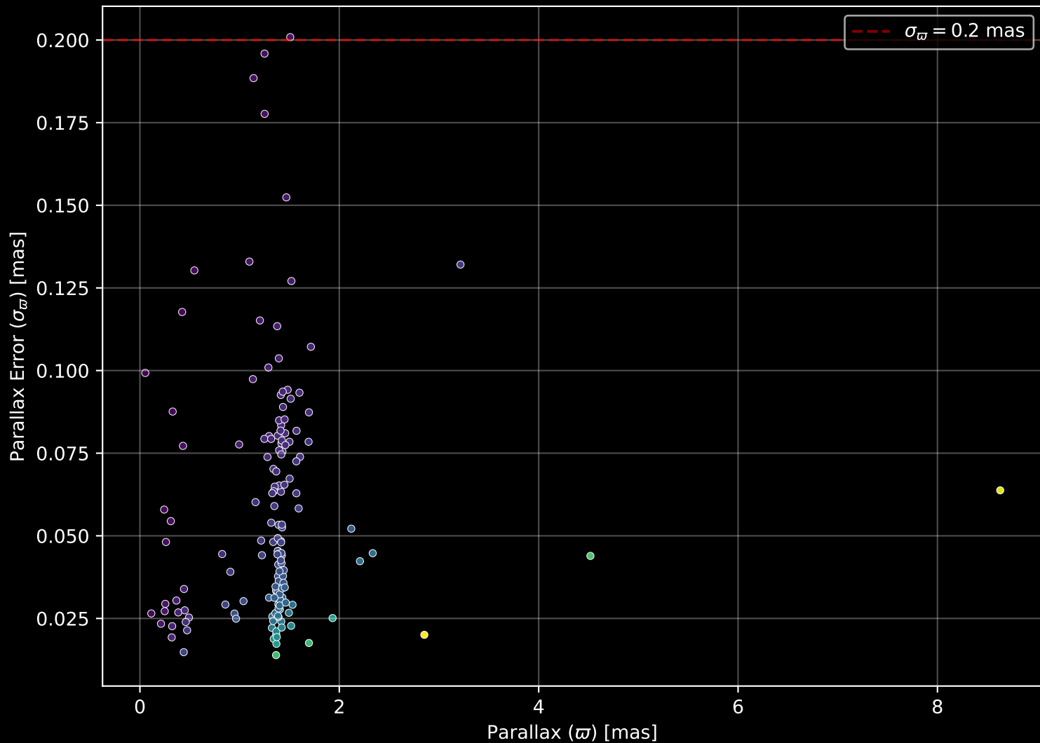
APOGEE DR17 Field: [N2264] Parallax Quality (n= 152)
