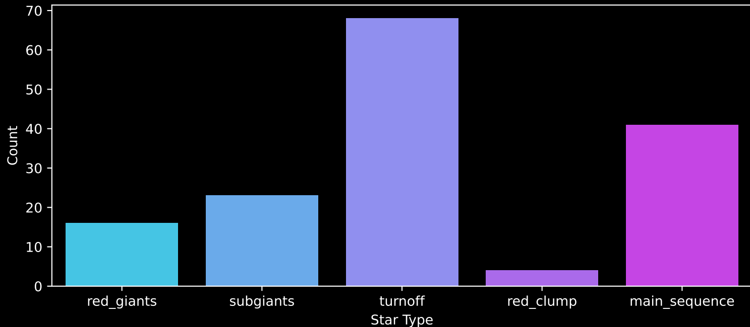
APOGEE DR17 Field: [N2264] Count plot of Star Type
