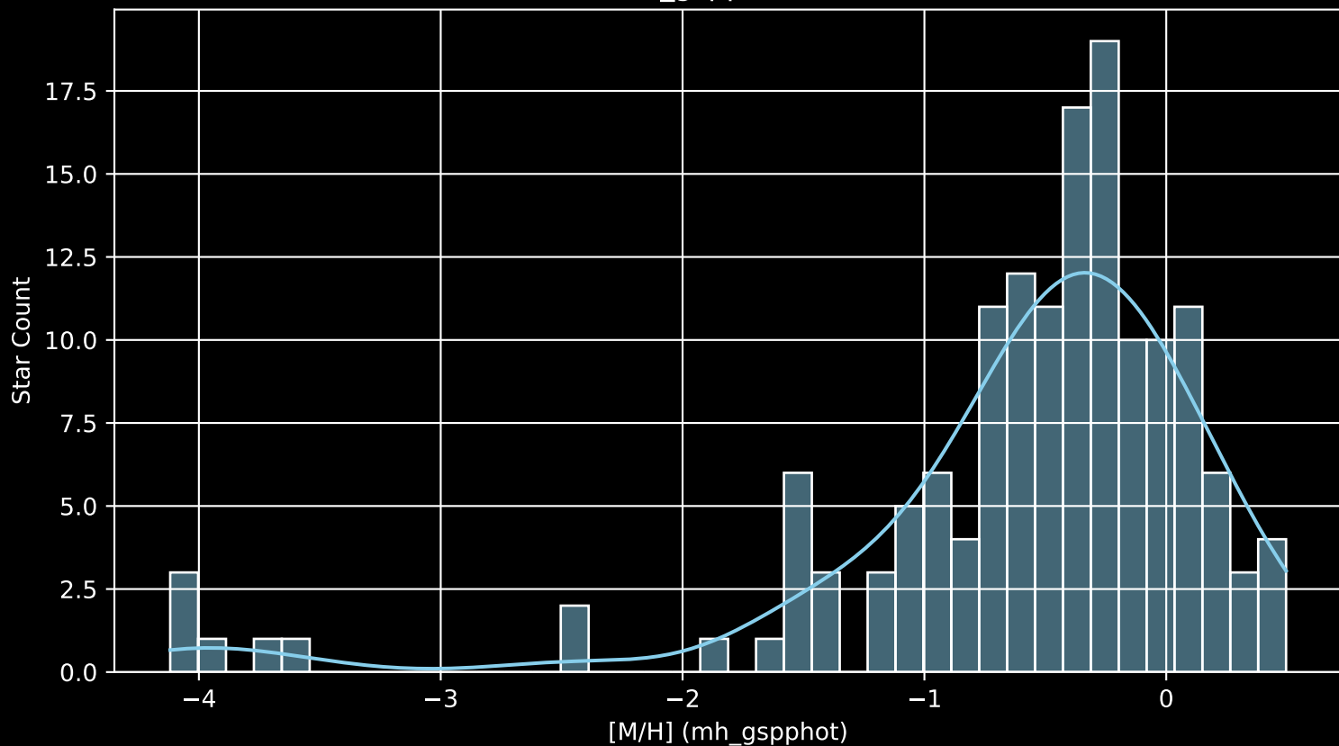
APOGEE DR17 Field: [N2264 [M/H] (mh_gspphot) (n= 151)
