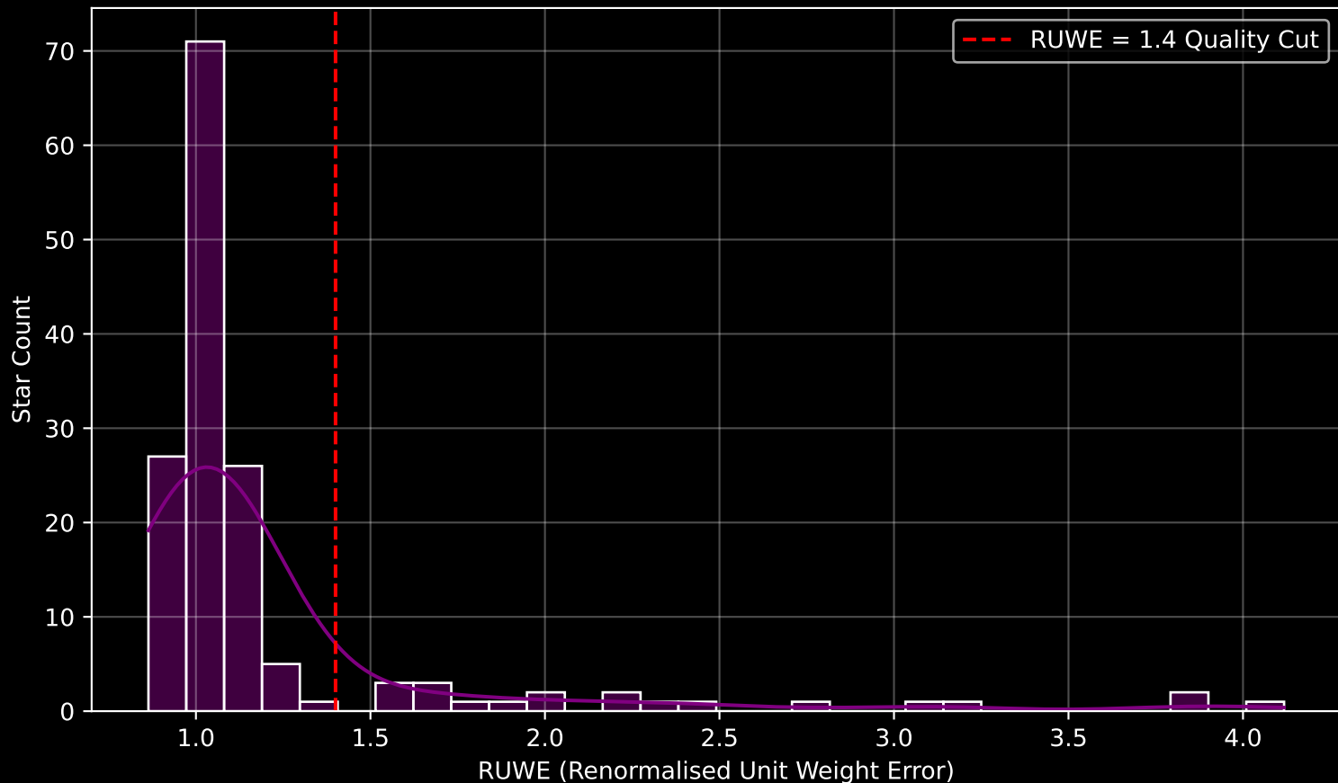
GAPOGEE DR17 Field [N2264] RUWE Distribution (n= 150)
