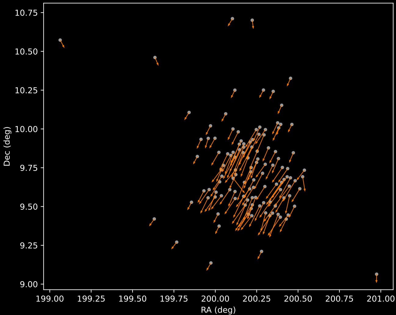
APOGEE DR17 Cluster 2 Proper Motion Vectors (n=119)
